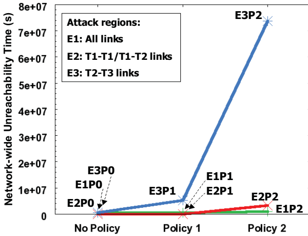
Fig. 24. Network-wide unreachability time plotted for all combinations of policy and attack topology.
