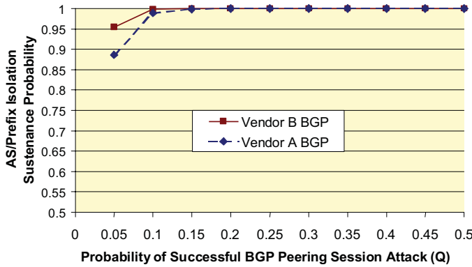
Fig. 11. Probability of sustenance of AS-prefix isolation as a function of success probability of peering session attack ( n = 4 ).
