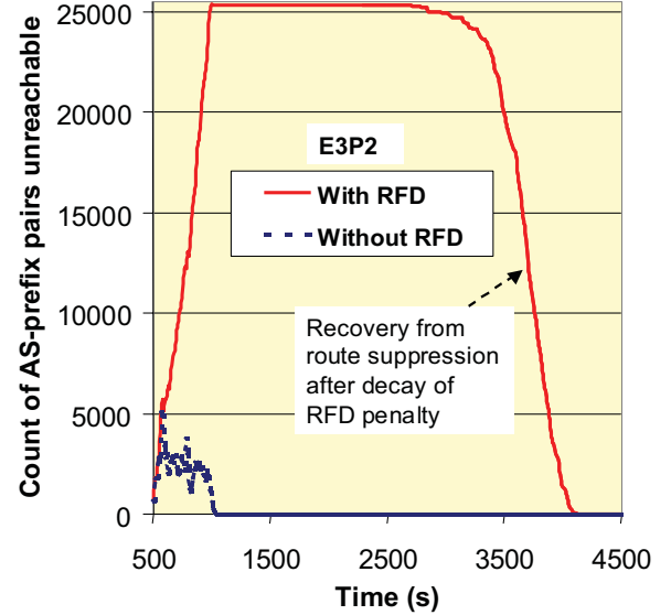
Fig. 21. Count of AS-prefix pairs unreachable as a function of time: comparison shows that unreachability gets much worse due to RFD.
